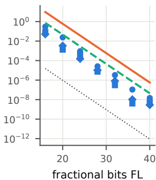
\partial V / \partial v_0
