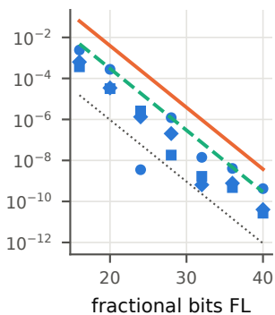
Delta \partial V / \partial S_0
