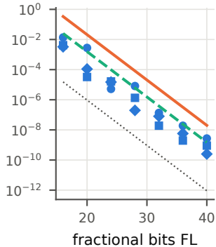
\partial V / \partial \rho
